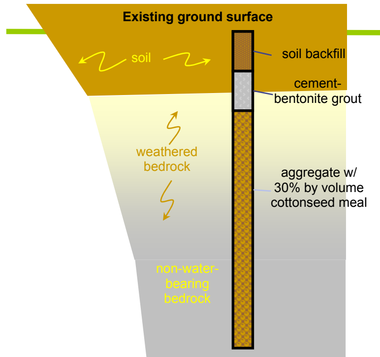
Figure A-32. Bioboring schematic.
