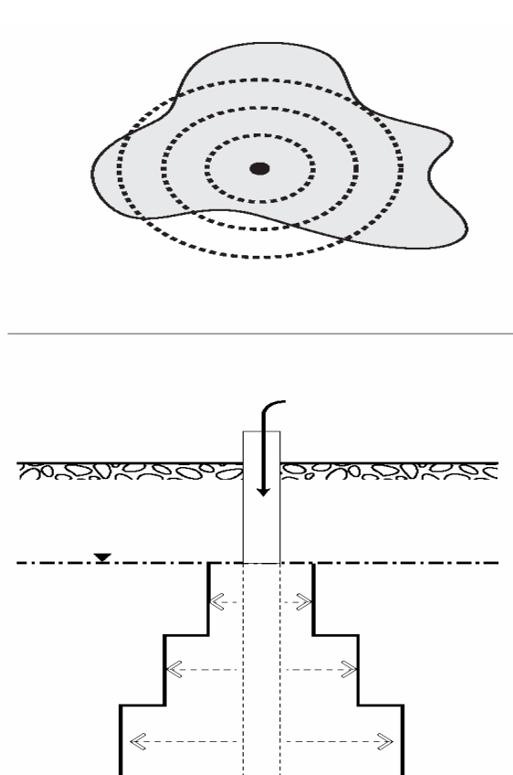
Figure 5-3. Bottom-up injections.
