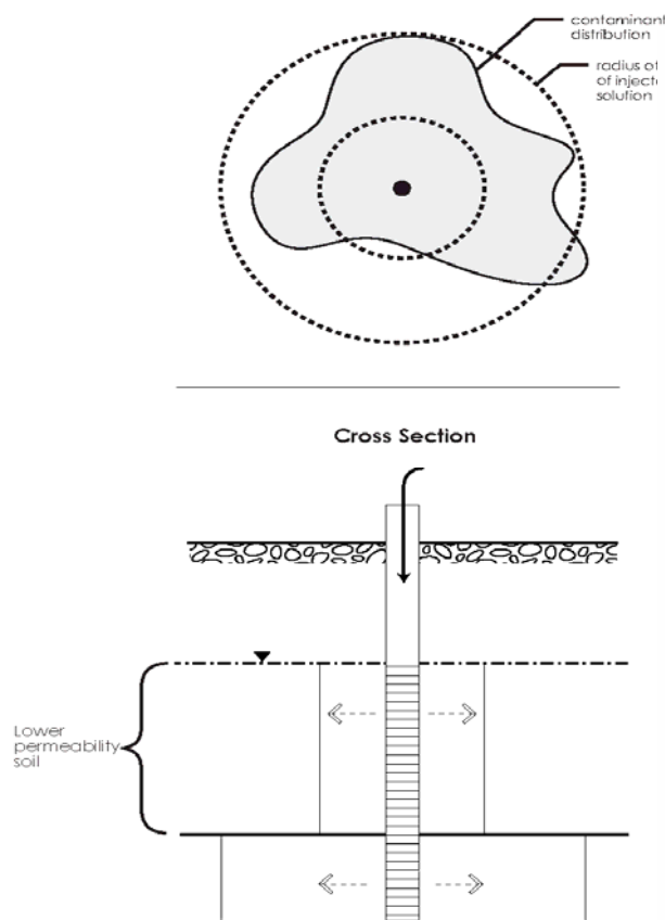
Figure 5-2. Permeability influences.
