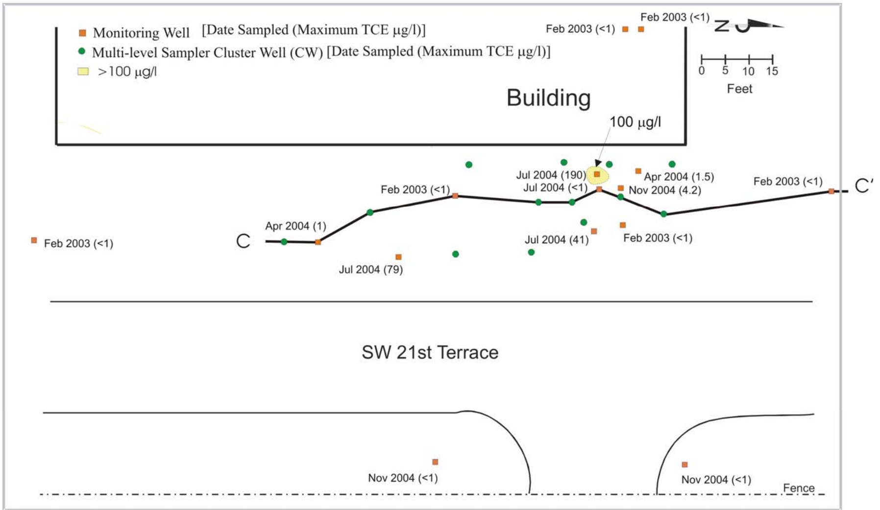
Figure 4. Plan view of TCE contamination after KMnO 4 injections (February 2003). Cross-section C-C' used in Figure 5.
