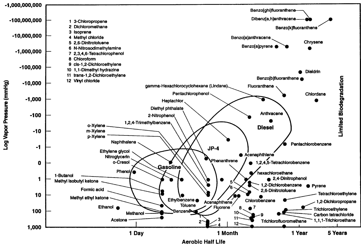
Figure 3-17. Relationship between contaminant pressure and aerobic biodegradability.
