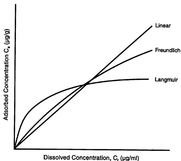
Figure 3-2. Sorption isotherms.
