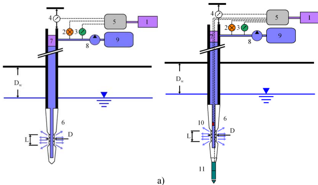
Figure 1. Perm  afor HPT test equipment (1: Laptop, 2: flow meter, 3: pressure sensor; 4: displacement transducer; 5: data logger, 6: Perm  afor tip; 7: water head; 8: pump; 9: water tank; 10: pressure transducer; 11: electric cone penetrometer with pore pressure measurement)
