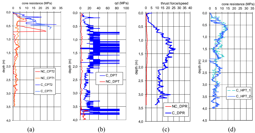
Figure 5 Profile (a) CPTu, (b) dynamy probing, (c) drilling parameter recording, (d) Permeafor CPT (C for compacted and NC for uncompacted cell)
