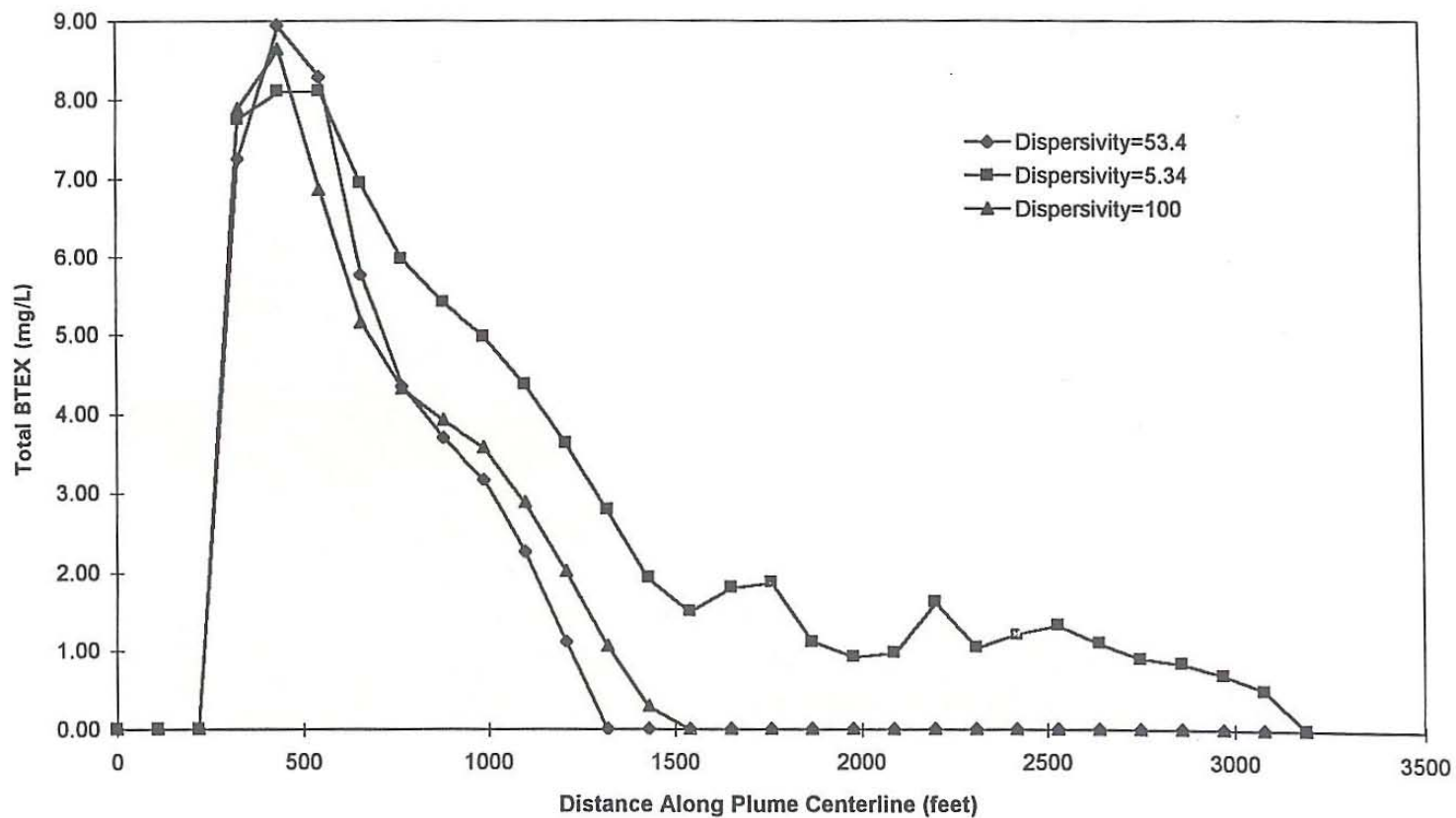
FIGURE 5.7 PLOT OF TOTAL BTEX VS DISTANCE ALONG PLUME CENTERLINE WITH VARYING DISPERSIVITY UST SITE 870 INTRINSIC REMEDIATION EE/CA HILL AFB, UTAH
