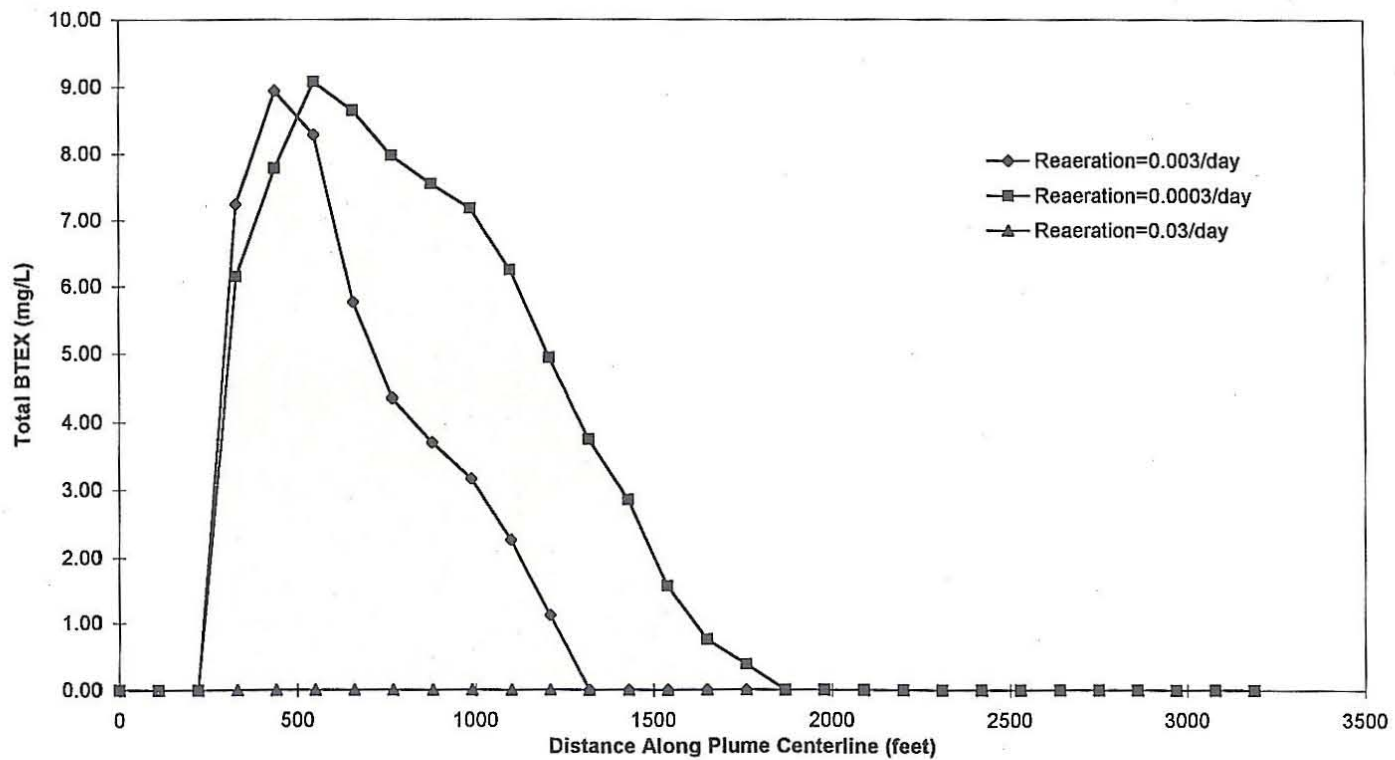
FIGURE 5.6 PLOT OF TOTAL BTEX VS DISTANCE ALONG PLUME CENTERLINE WITH VARYING COEFFICIENT OF REAERATION UST SITE 870 INTRINSIC REMEDIATION EE/CA HILL AFB, UTAH
