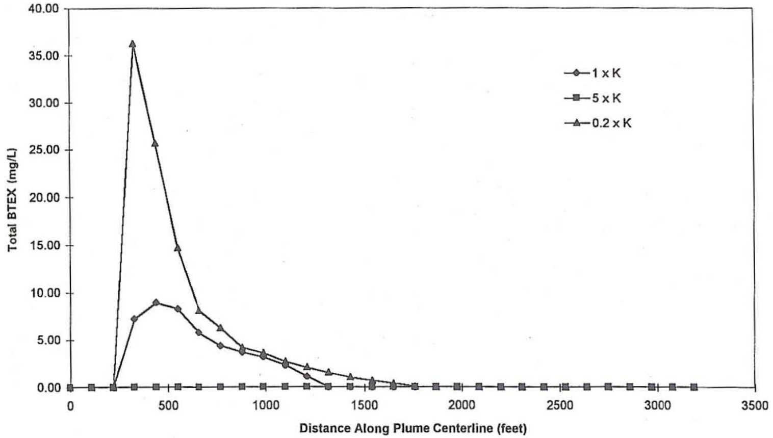
FIGURE 5.5 PLOT OF TOTAL BTEX VS DISTANCE ALONG PLUME CENTERLINE WITH VARYING HYDRAULIC CONDUCTIVITY UST SITE 870 INTRINSIC REMEDIATION EE/CA HILL AFB, UTAH
