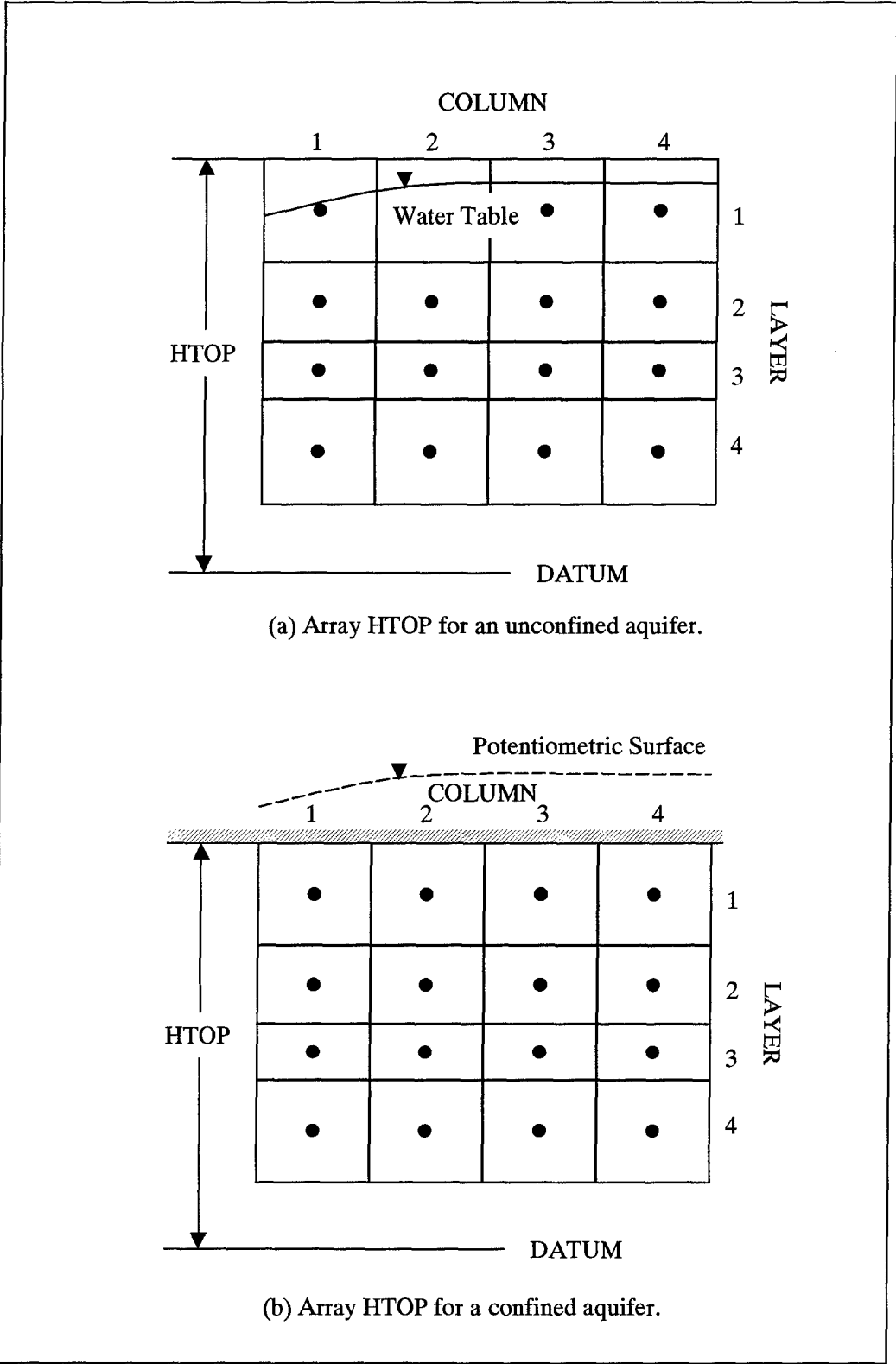
Figure 27. Illustration of array HTOP for (a) unconfined and (b) confined aquifer layers
